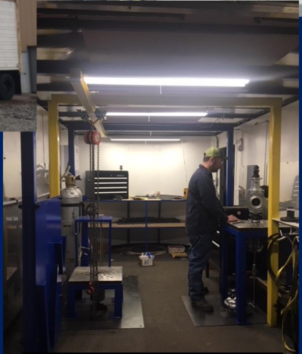
Mobile Valve Test Stand
