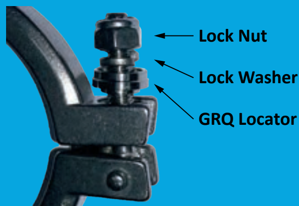
GRQ-LL ENGINEERED CLAMP for THERMAL CYCLING or VIBRATION
