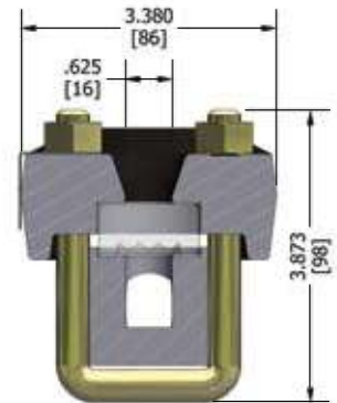
Series R-20 Reflex
