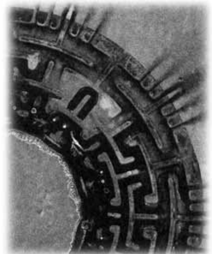
TEST CASE SHOWING SEVERE BLOCKAGE. ALL INLETS AND OUTLETS STILL IN USE. NEGLIGIBLE LOSS IN CV.
